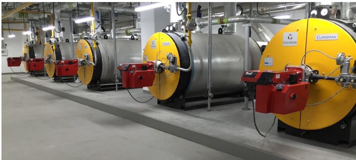
Typical hot water boiler installation Image courtesy of Cochran Ltd
